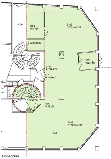
Bottenplan
